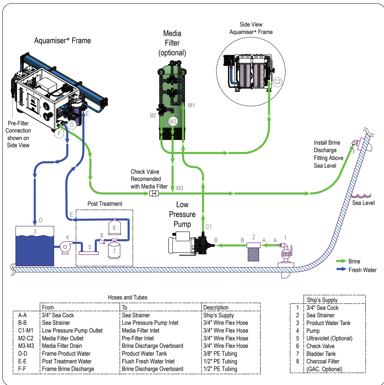
Figure 16: Plumbing Diagram (layout with dual pre-filter/media filter)
