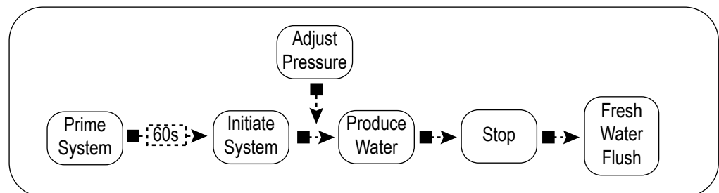
Figure 27: Operation Cycle
