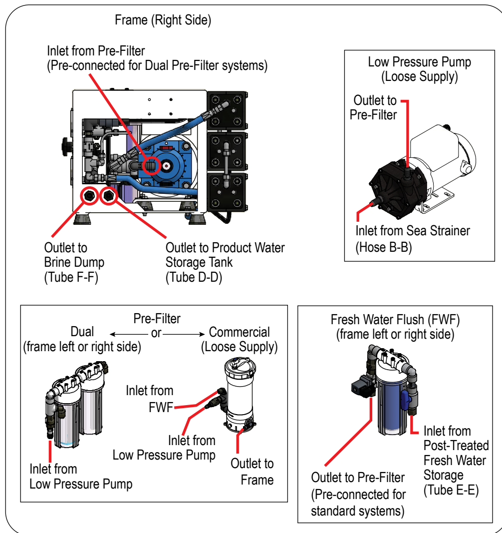
Figure 20: Plumbing Connections
