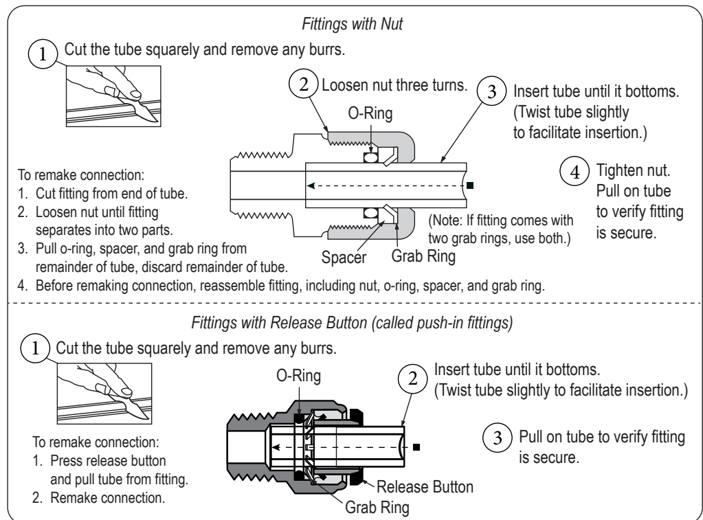
Figure 19: Proper Tube Fitting and Hose Connections
