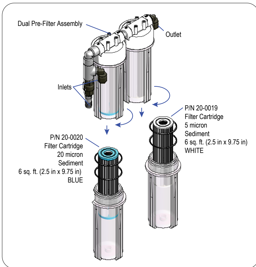
Figure 46: Replacing Dual Pre-filter Elements
