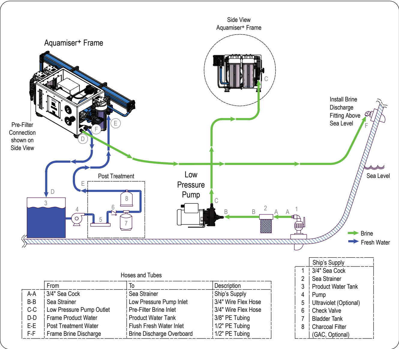
Figure 15: Plumbing Diagram (layout with dual pre-filter)
