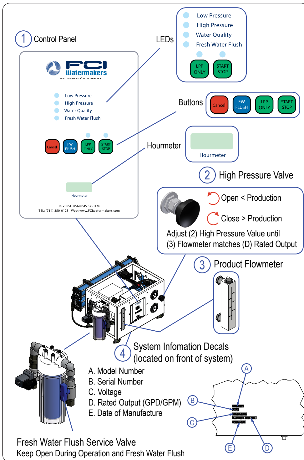
Figure 26: Operational Controls
