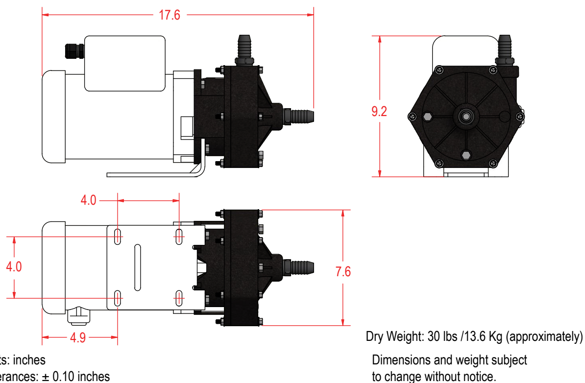
Figure 13: Dimensions, Weight & Footprint for Low Pressure Pump (1-phase)
