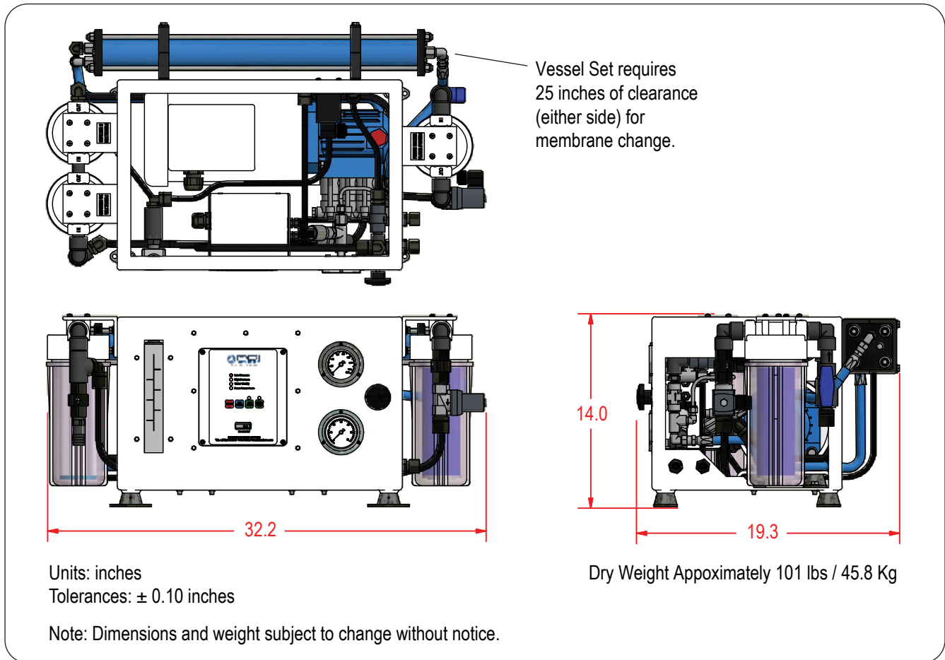
Figure 6: Dimensions & Weight for Standard 250 GPD System
