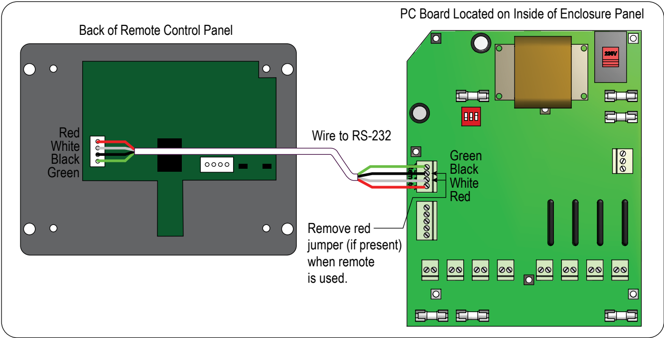
Figure 24: Remote Control Panel Wiring
