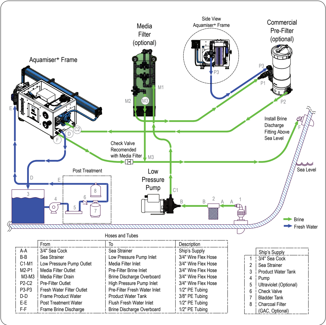
Figure 18: Plumbing Diagram (layout with commercial pre-filter/media filter)
