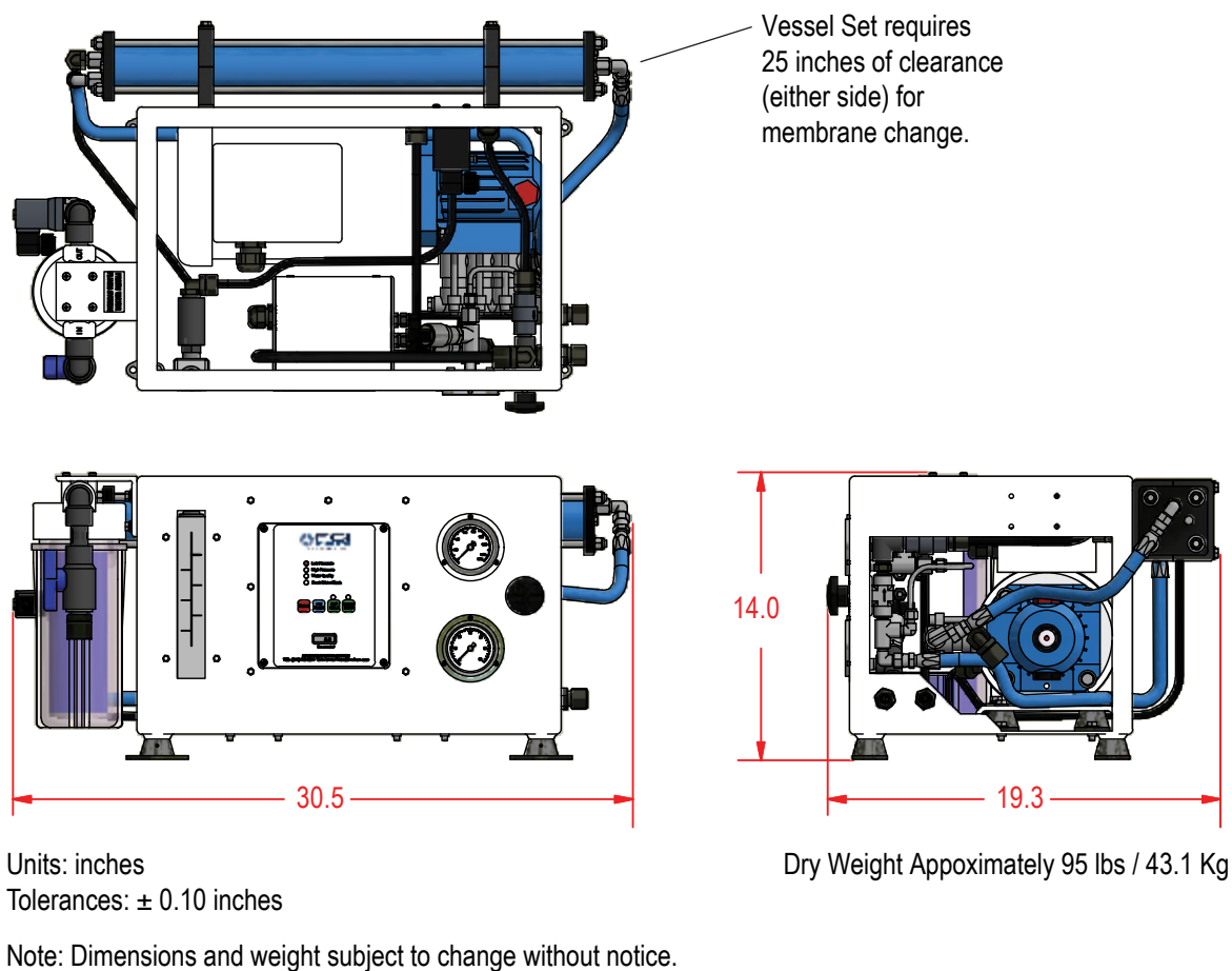
Figure 7: Dimensions & Weight for Commercial 250 GPD System
