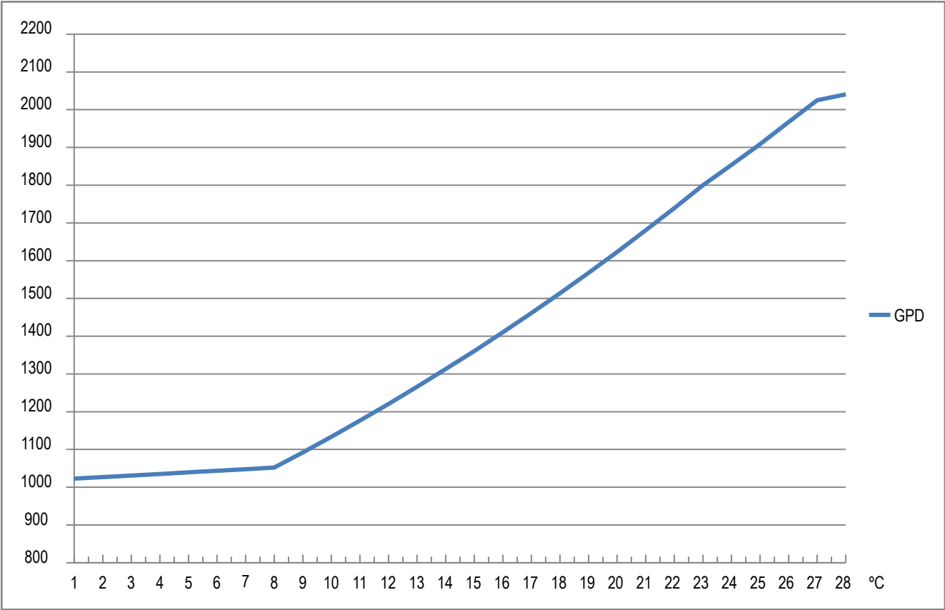
Figure 25: Water Temperature vs. Output (constant pressure)
