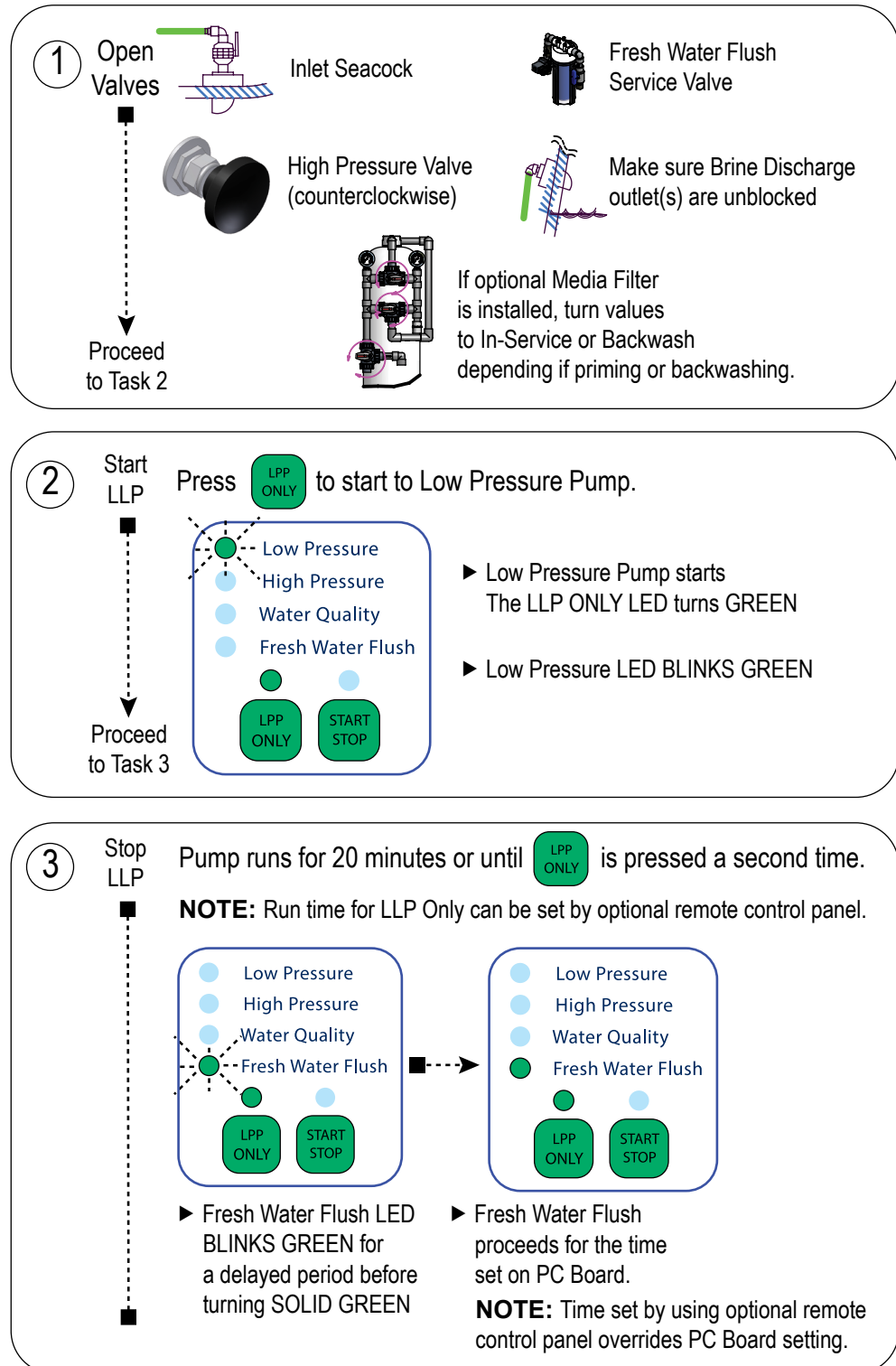
Figure 37: Manual Low Pressure Pump Operation
