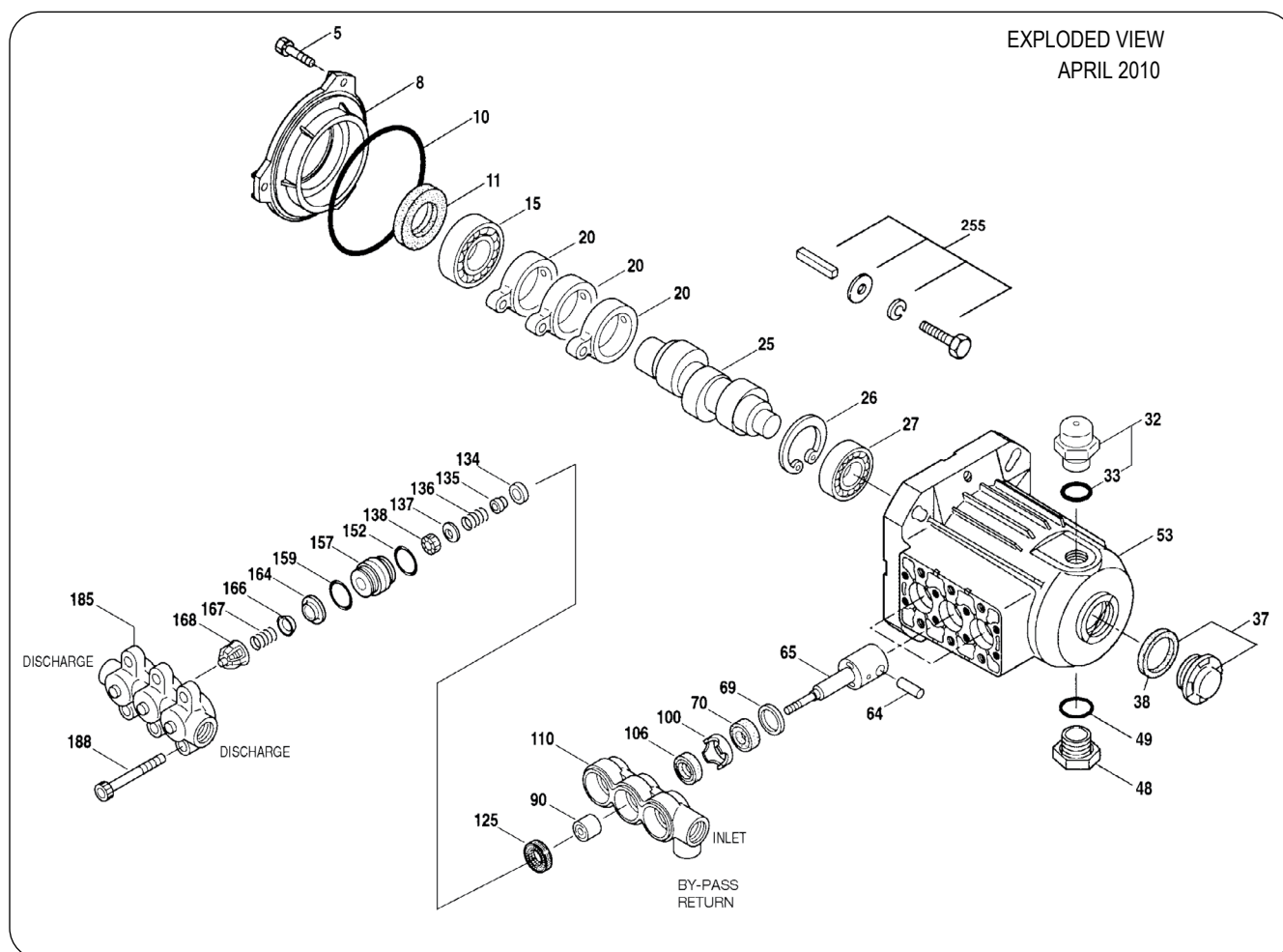
Figure 49: High Pressure Pump Exploded View
