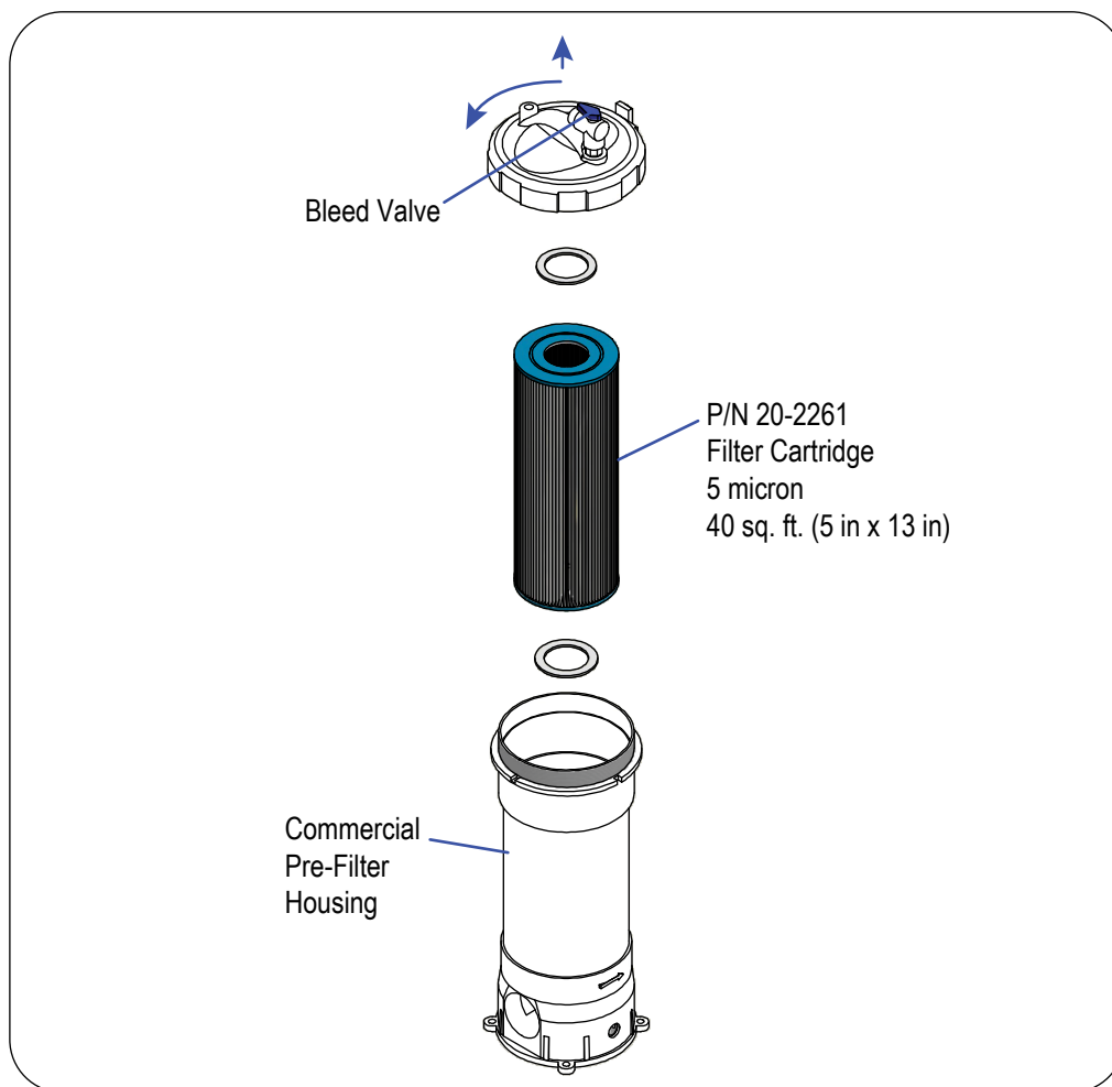
Figure 47: Replacing Commercial Pre-filter Element
