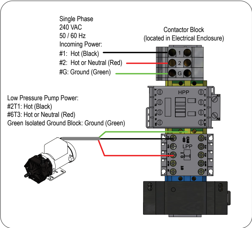
Figure 23: Wiring at the Contactor Block (240 VAC)
