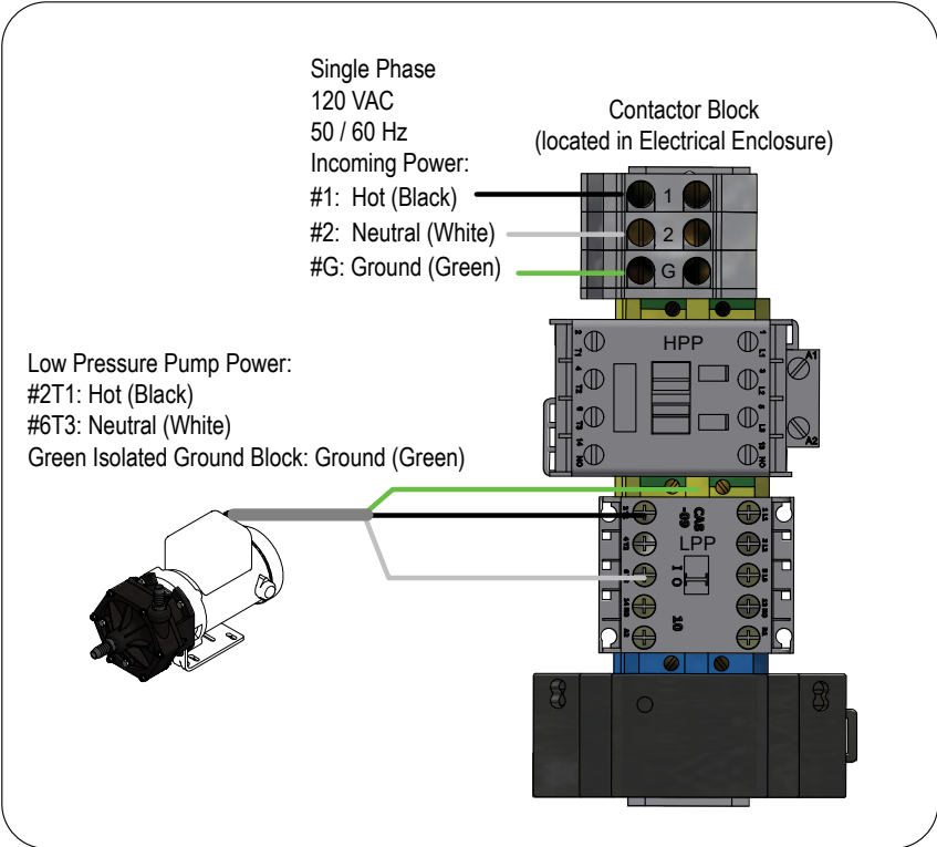
Figure 22: Wiring at the Contactor Block (120 VAC)
