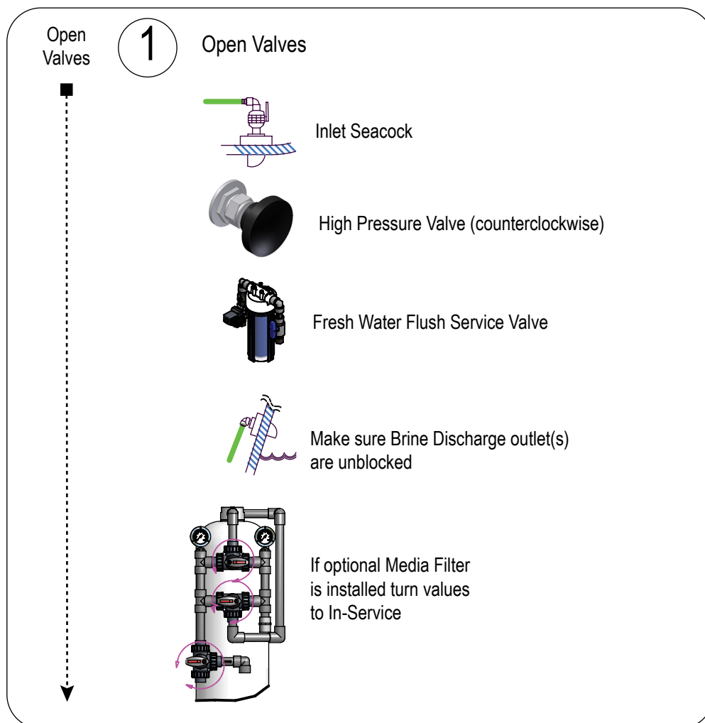
Figure 30: Quick Start and Stop Task 1 (open all valves)
