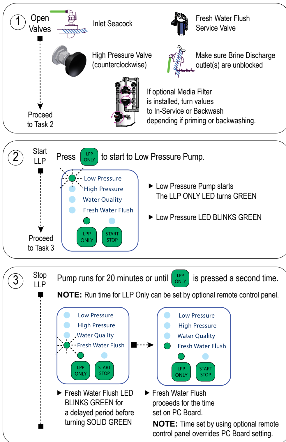
Figure 46: Manual Low Pressure Pump Operation
