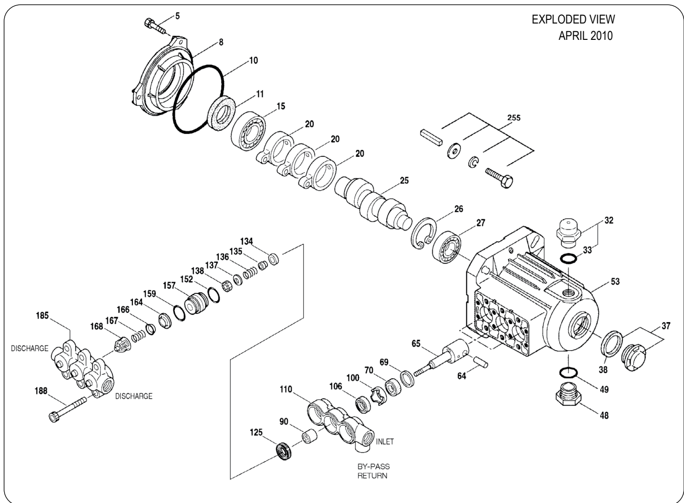
Figure 58: High Pressure Pump Exploded View
