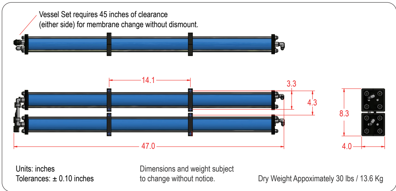
Figure 9: Dimensions & Weight for 800 and 1,200 GPD Pressure Vessel Assembly
