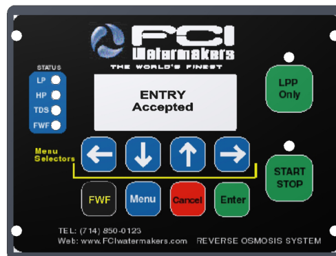
Figure 53: Remote Menu Screen
