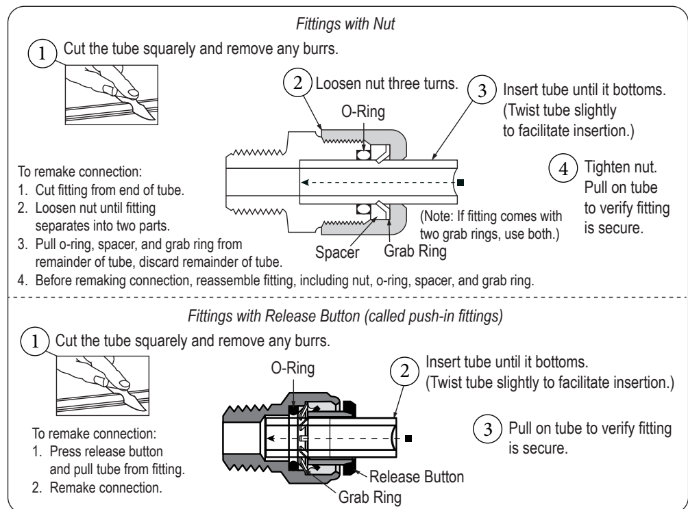
Figure 24: Proper Tube Fitting and Hose Connections
