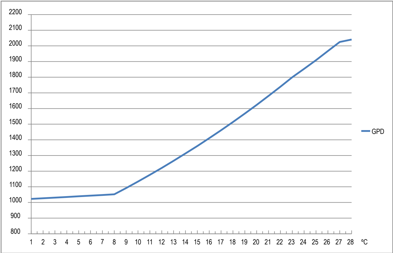
Figure 34: Water Temperature vs. Output (constant pressure)
