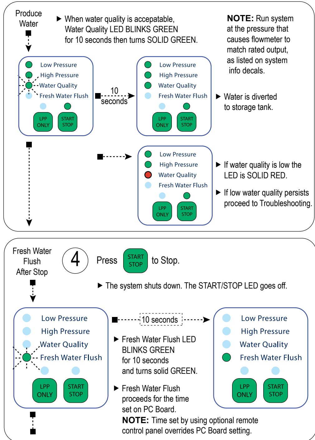
Figure 42: Quick Start and Stop Task 4 (press start/stop button to stop)
