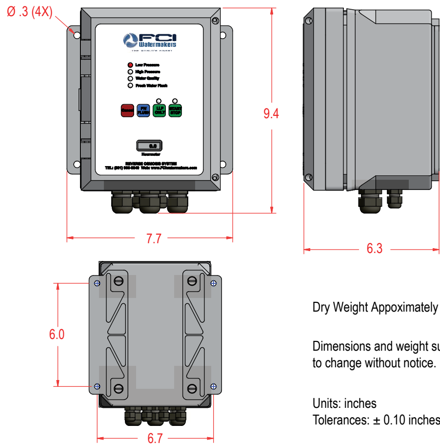
Figure 15: Dimensions, Weight & Footprint for Electronics Enclosure
