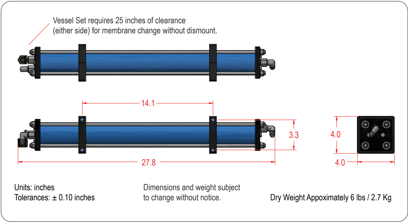
Figure 6: Dimensions & Weight for 250GPD Pressure Vessel Assembly
