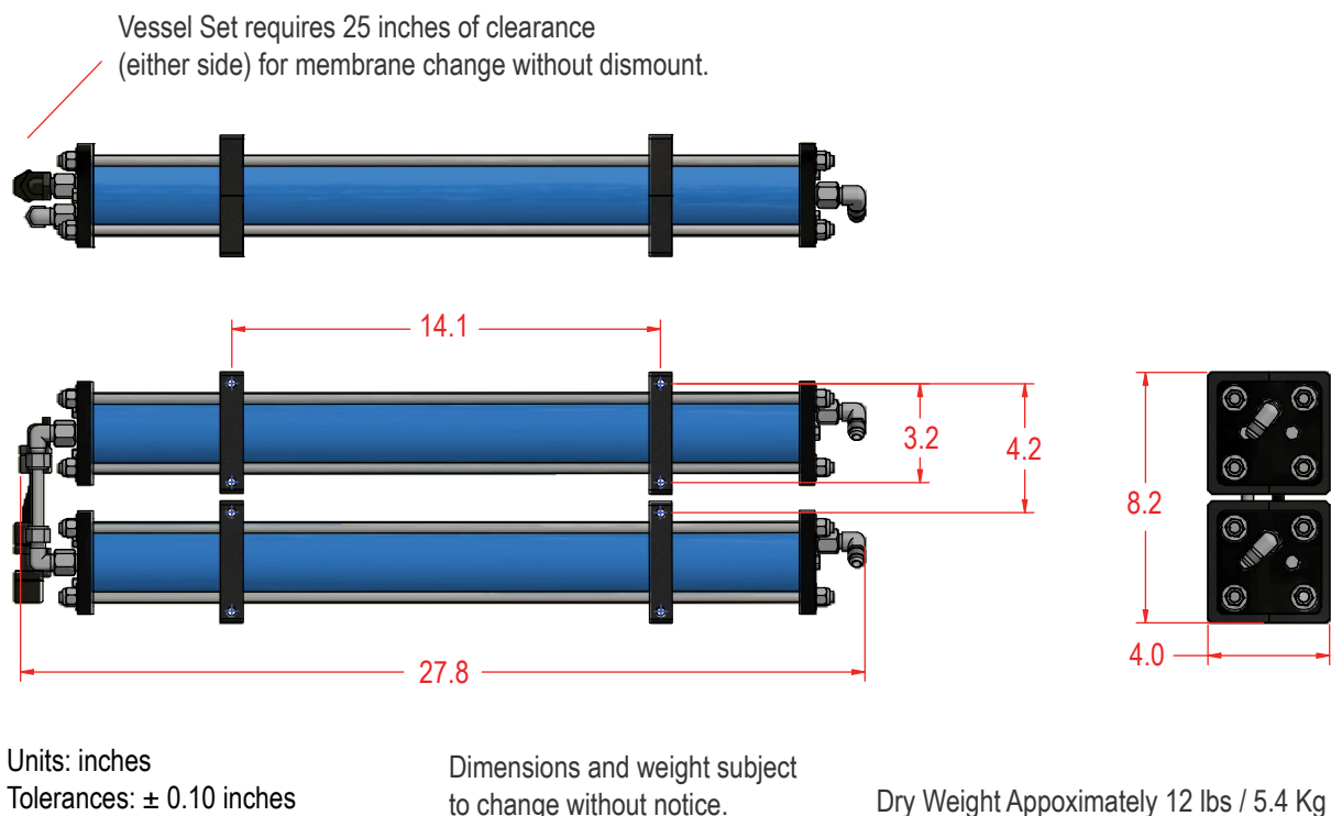
Figure 7: Dimensions & Weight for 500 GPD Pressure Vessel Assembly
