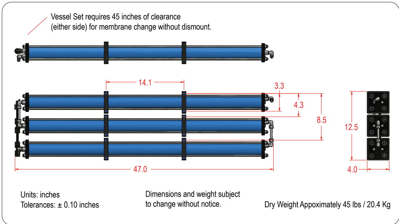
Figure 10: Dimensions & Weight for 1,800 GPD Pressure Vessel Assembly
