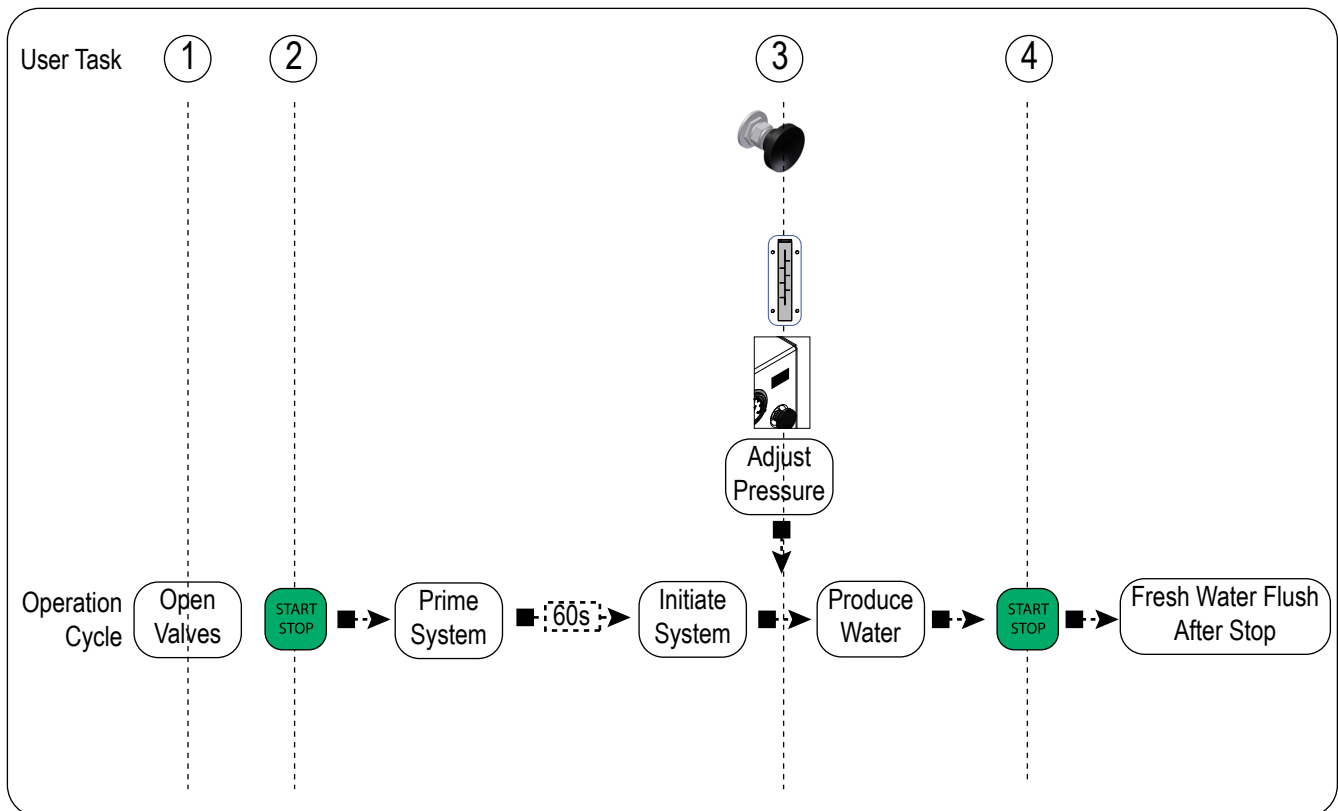
Figure 38: Overview of Quick Start and Stop
