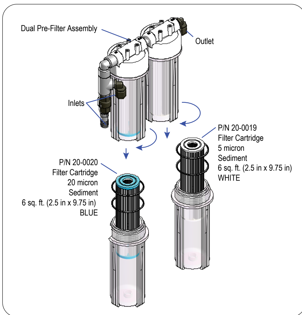
Figure 55: Replacing Dual Pre-filter Elements
