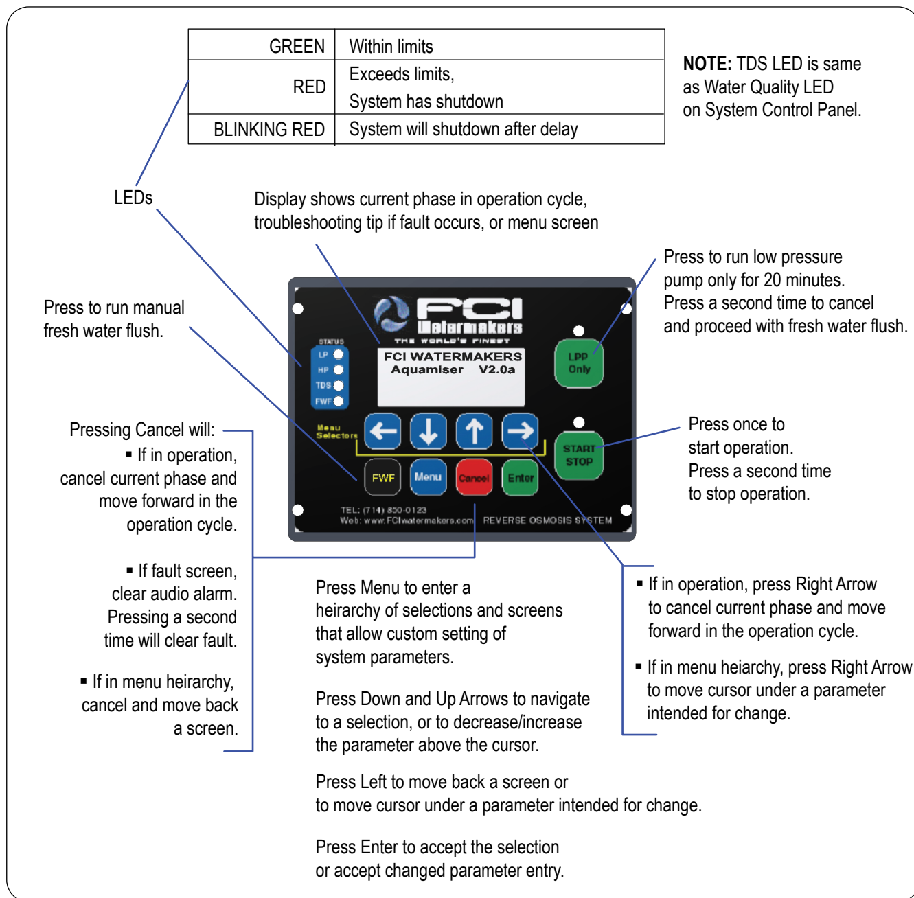
Figure 48: The Remote Control Panel
