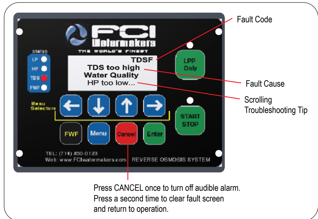
Figure 61: Remote Control Fault Codes
