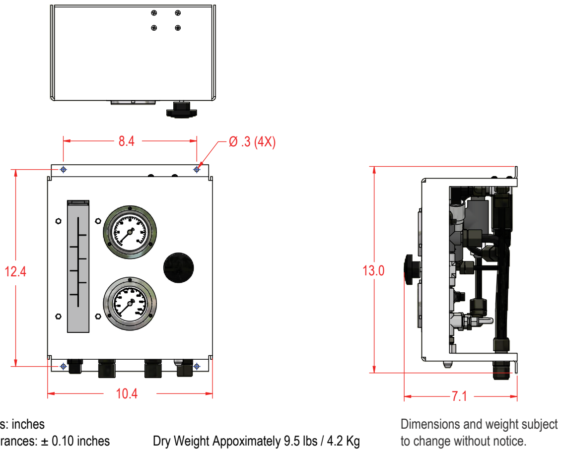
Figure 14: Dimensions, Weight & Footprint for Flow Control Panel
