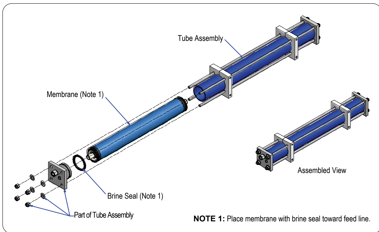
Figure 60: Replacing the Membrane
