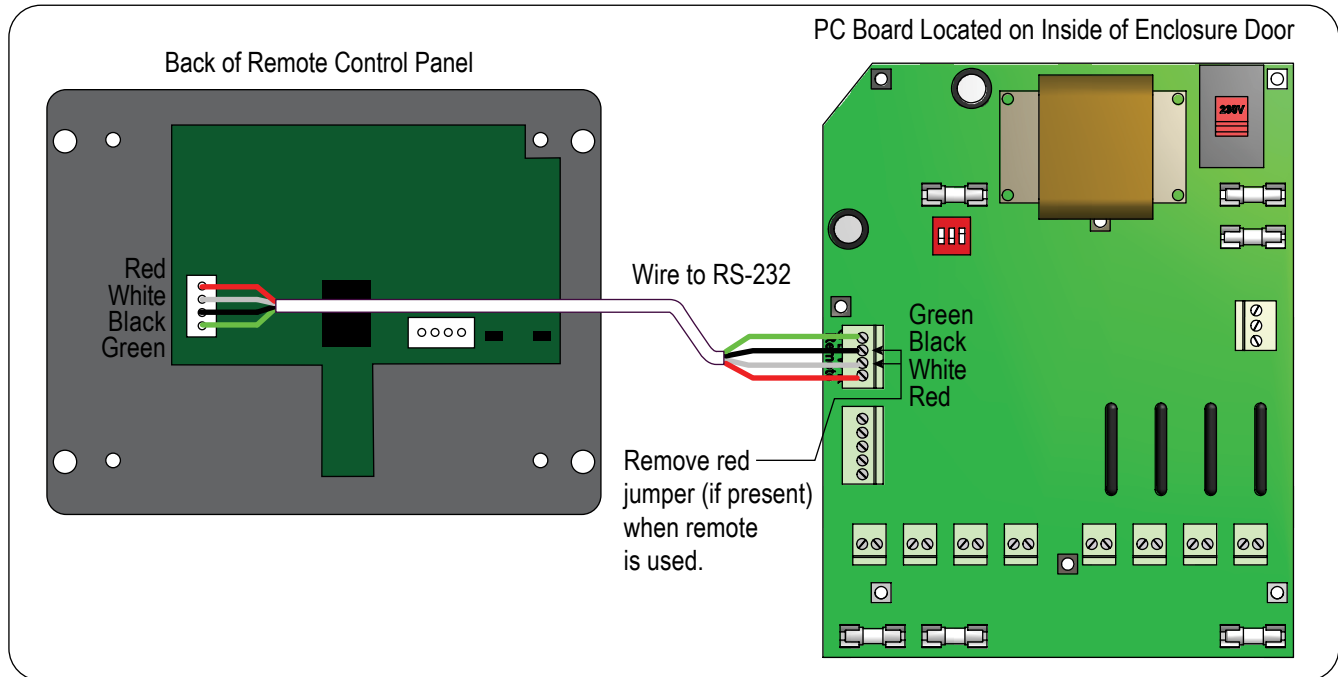
Figure 33: Remote Control Panel Wiring
