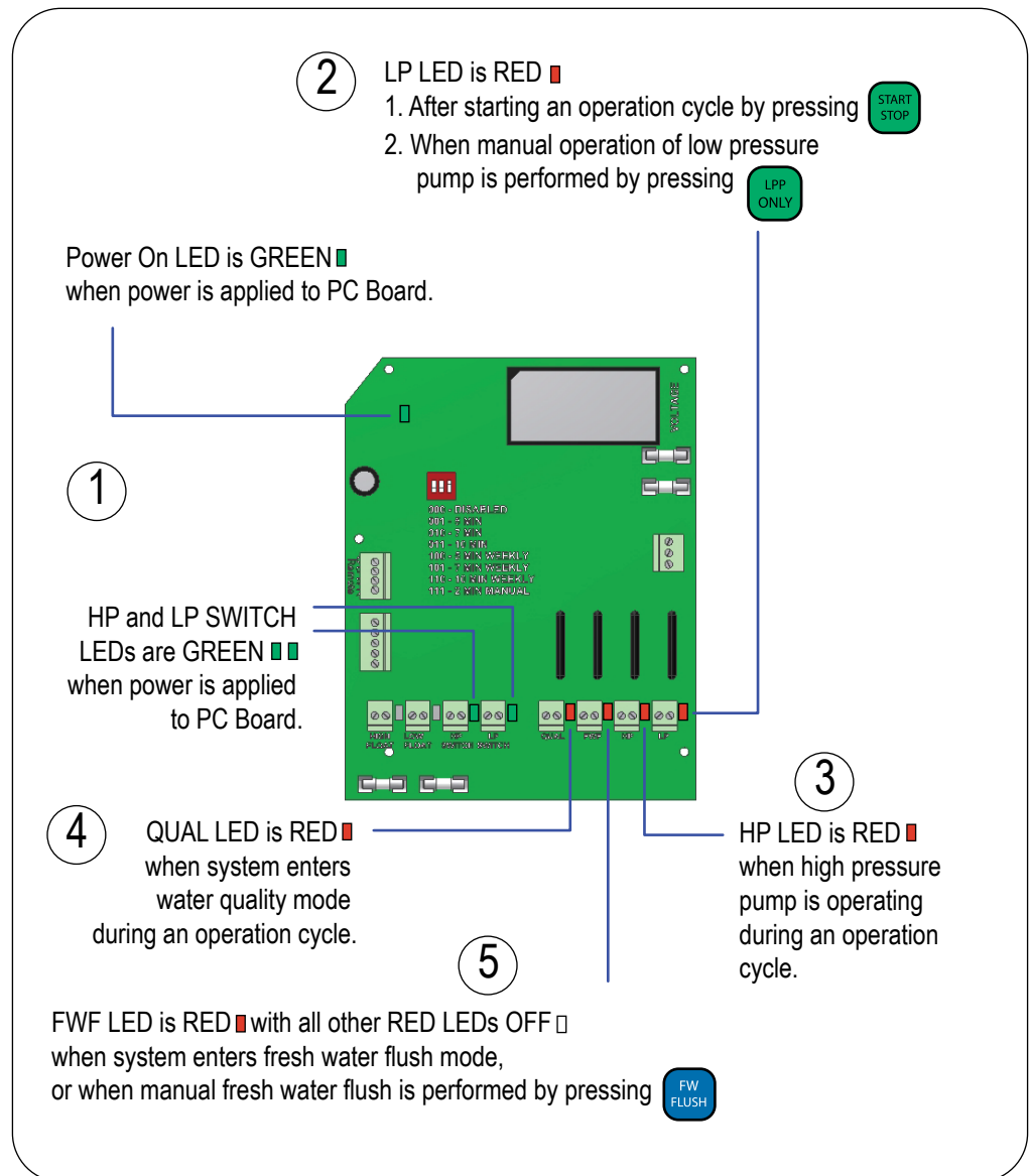
Figure 47: PC Board LED Indicators
