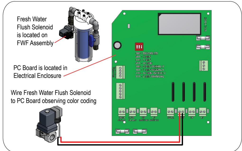
Figure 29: Wiring the FWF Solenoid
