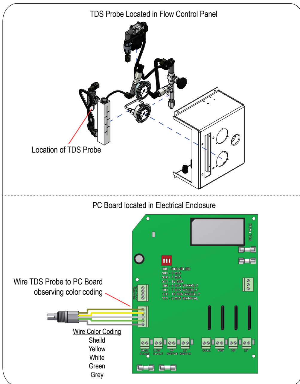
Figure 32: Wiring the TDS Probe
