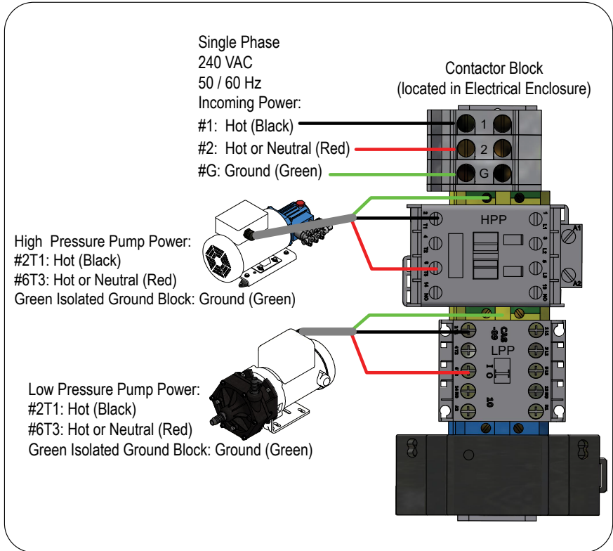
Figure 28: Wiring at the Connector Block (240VAC)
