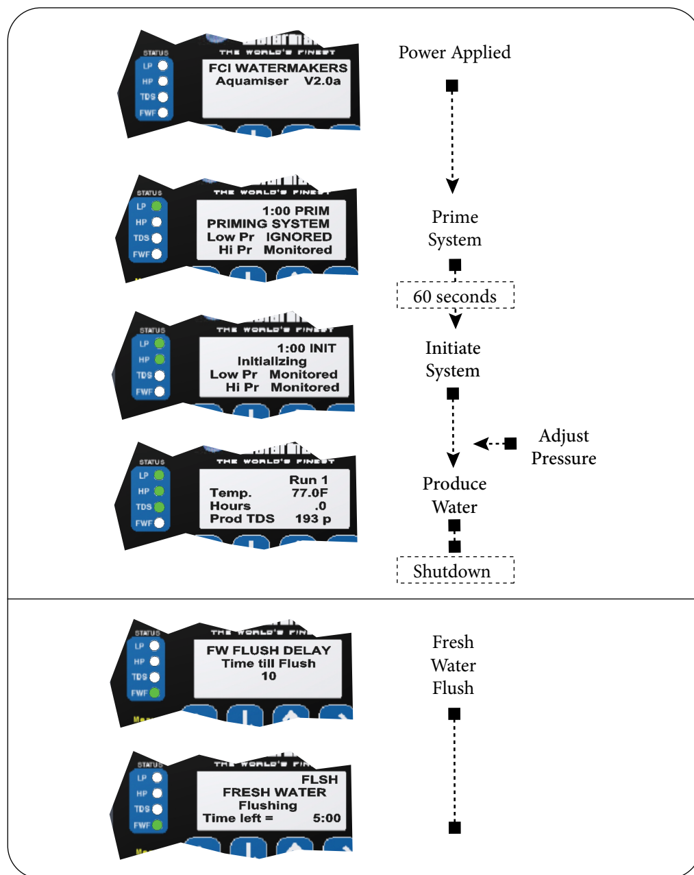
Figure 49: The Remote Control Display in an Operation Cycle
