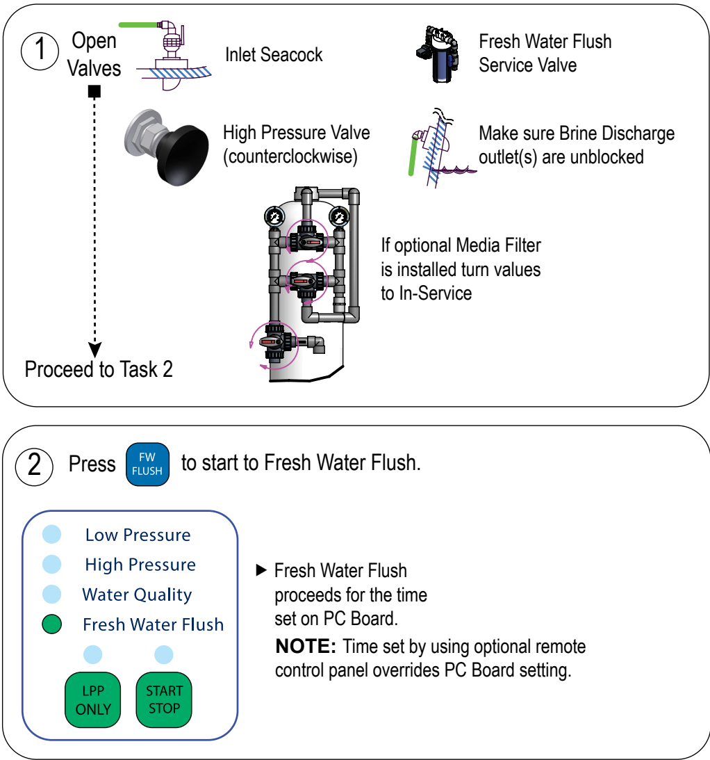
Figure 45: Manual Fresh Water Flush
