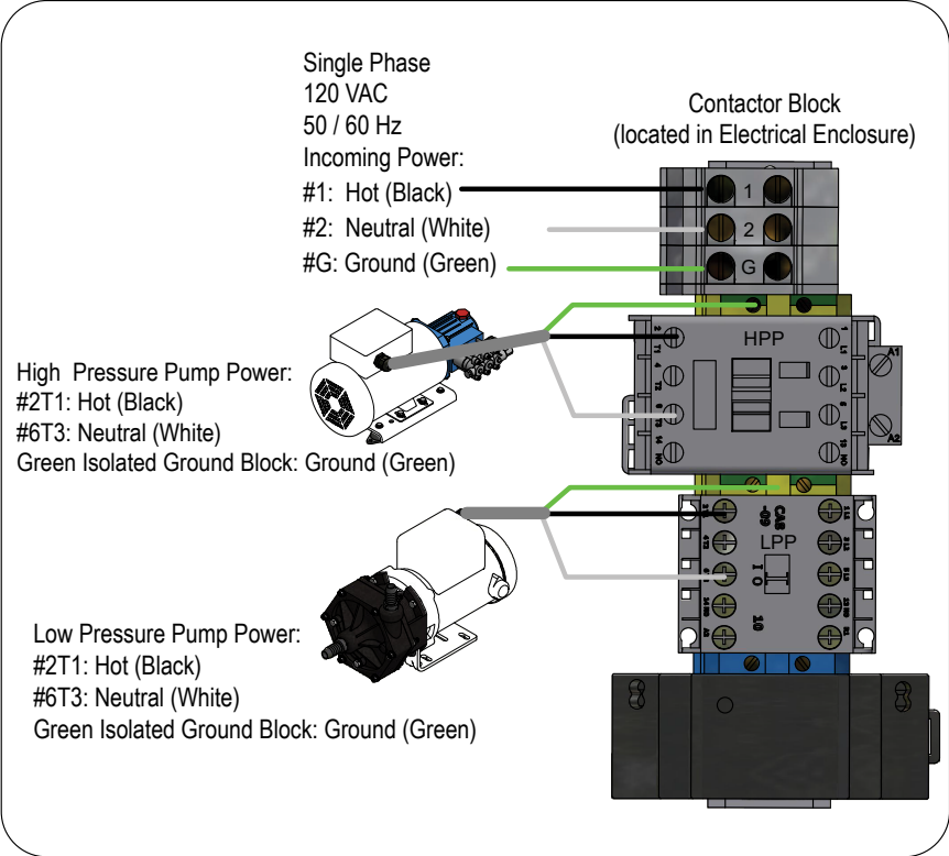
Figure 27: Wiring at the Connector Block (120VAC)
