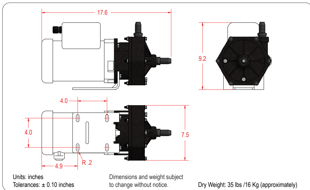
Figure 13: Dimensions, Weight & Footprint for Low Pressure Pump (single phase)
