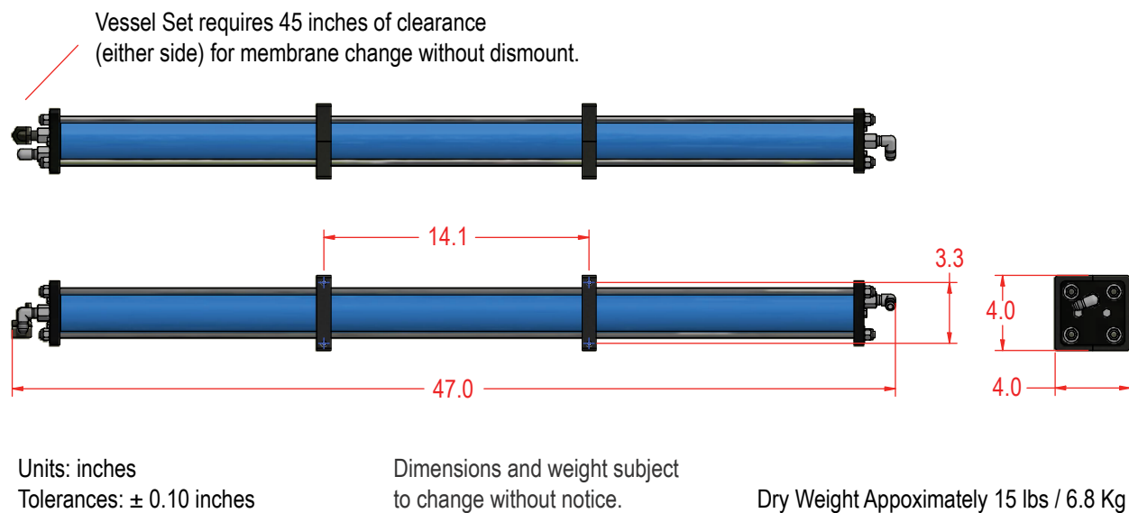
Figure 8: Dimensions & Weight for 600 GPD Pressure Vessel Assembly
