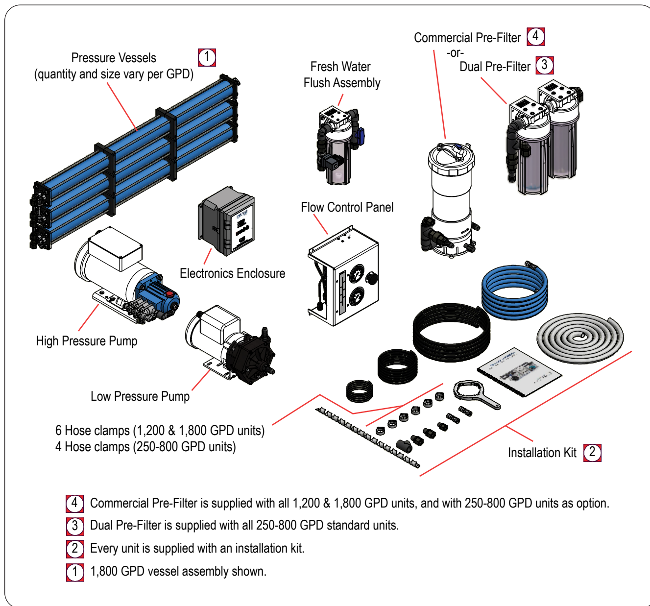
Figure 2: System Components Identification
