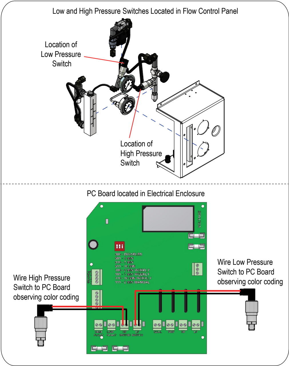
Figure 31: Wiring the LP and HP Pressure Switches
