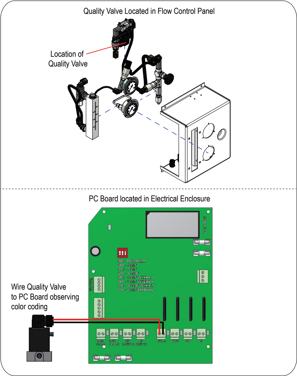
Figure 30: Wiring the Quality Valve
